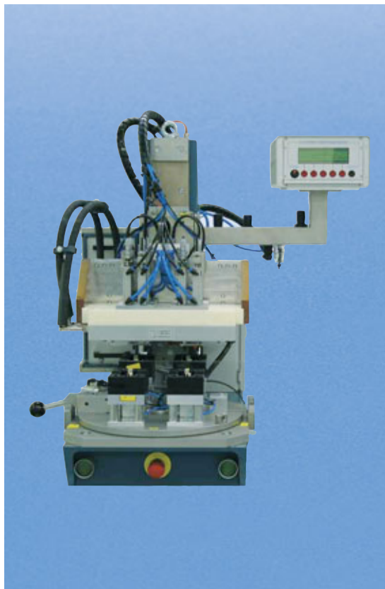
ERW thermal installation machine to embed eight inserts M 1.6 into two mobile phone half shells
